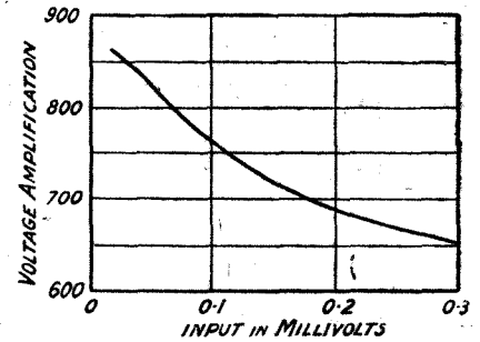
Fig. 4.—From the curve of a 6-valve untuned transformer-coupled amplifier it appears that the amplification falls with increasing input.
