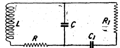
Fig. 5.—Showing how an amplifier has the effect of adding a shunt resistance and capacity across a tuned circuit.
