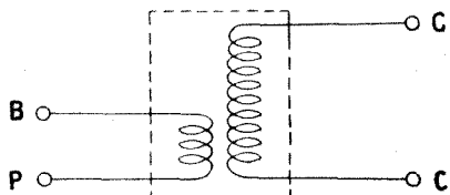
Fig. 4.—Showing the correct method of connection for the ends of the H.F. transformer windings.
