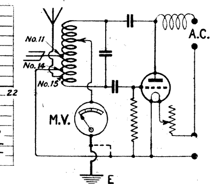
Figs. 3a and 3b.—Further readings were taken on the circuit of Fig. 2b, with the addition of the aerial system.
